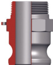
Type F male NPT x male adapter
