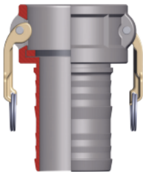
Type C female coupler x hose shank
