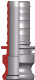
Type E male adapter x hose shank
