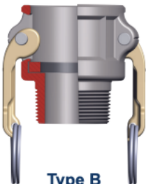
Type B female coupler x male NPT
