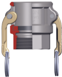
Type D female coupler x female NPT
